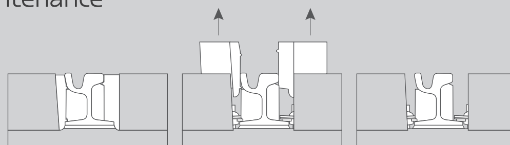
Vertical extraction and replacement of the pieces without requiring demolition of the track covering
