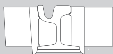
Full assembly
