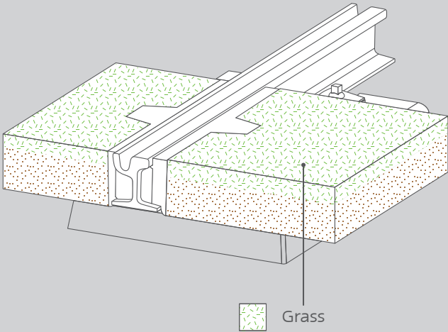
Green track No steel profiles
